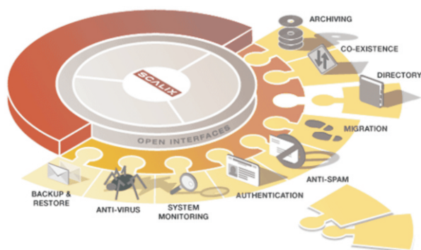
Scalix Architecture
